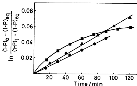
Fig. 1. Isomerization of 1-pentene catalyzed by NiX-(PPh 3 ) 3 .
